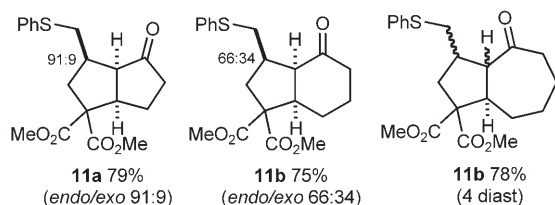
Scheme 10. Fused bicyclic ketones.
