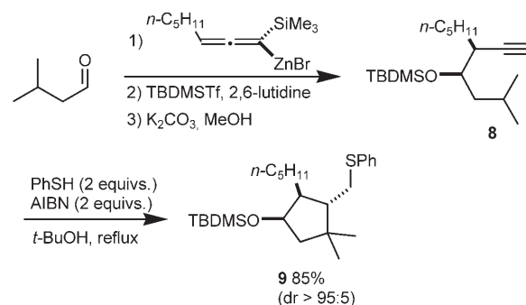
Scheme 9. Effect of vicinal substituents.
