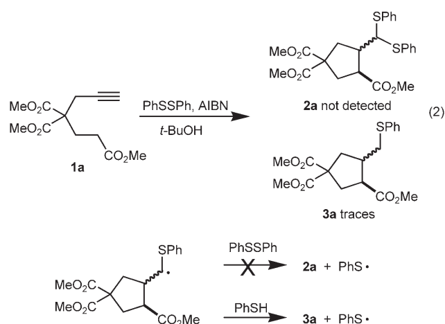
Scheme 2. Attempt to develop a diphenyl disulfide-mediated reaction.
