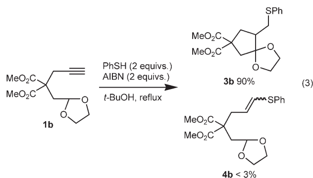
Scheme 3. Optimization of the reaction conditions with thiophenol.
