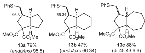
Scheme 11. Fused bicyclic alkanes.
