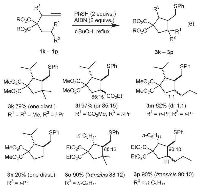
Scheme 7. Effect of the substitution at the propargylic center.
