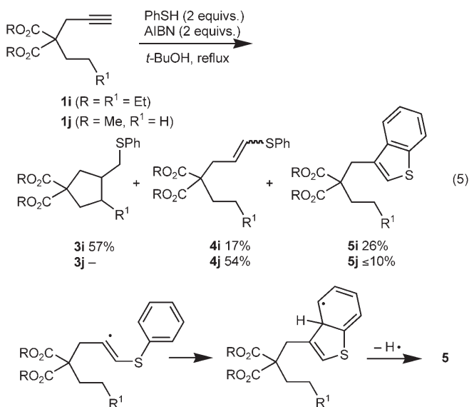
Scheme 6. Limitation of the method: formation of reduced products and benzothiophene derivatives.
