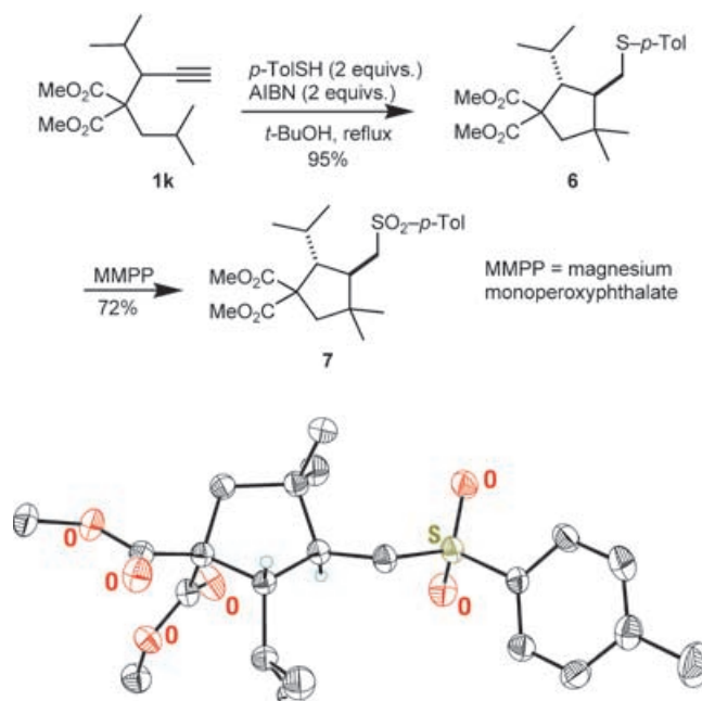
Scheme 8. Determination of the relative configuration of 7 by X-ray crystal structure analysis.
