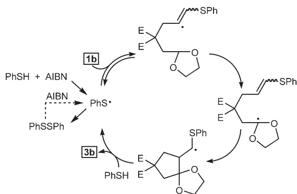
Scheme 4. Proposed mechanism.
