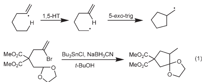
Scheme 1. 1,5-Hydrogen transfer-cyclization process.
