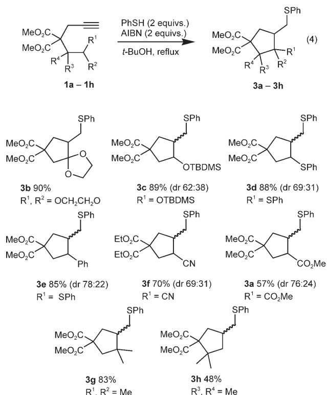
Scheme 5. Reaction with propargylmalonate derivatives.
