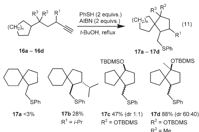
Scheme 13. Spirocyclic alkanes.
