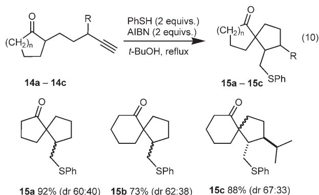
Scheme 12. Spirocyclic ketones.
